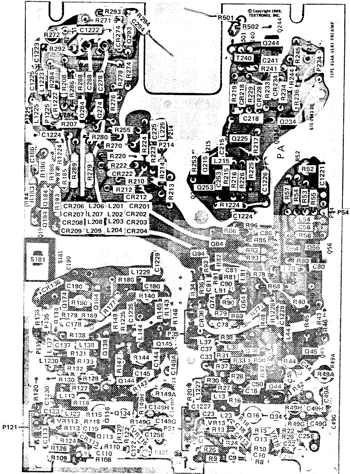
Fig. 8-3. Partial Vertical Preamp circuit board—P/O A1. Vertical Switching circuit shown.
