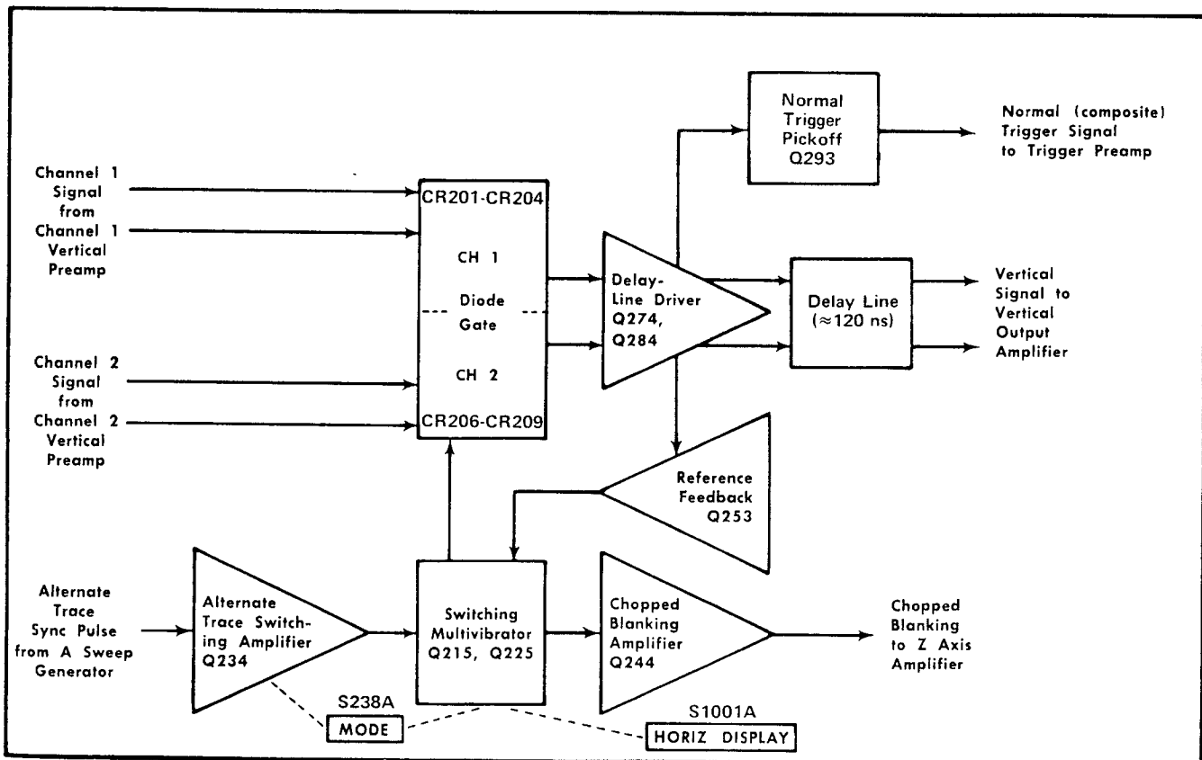
Fig. 3-4. Vertical Switching detailed block diagram.
